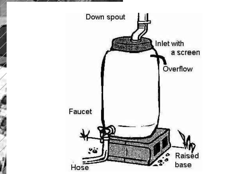
TYPICAL RAIN BARREL DETAIL NO SCALE
