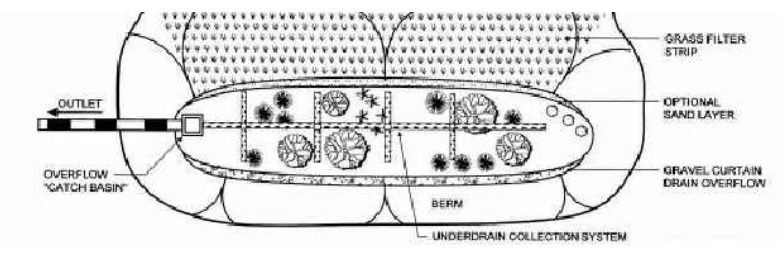
TYPICAL BIORETENTION AREA DETAIL NO SCALE
