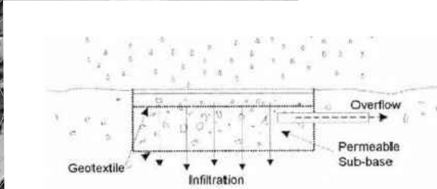
TYPICAL PERVIOUS PAVEMENT DETAIL NO SCALE
